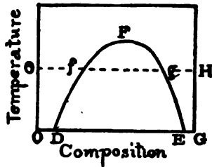
Fig. 43. Saturation-point Curve of Molten Binary Alloys.
